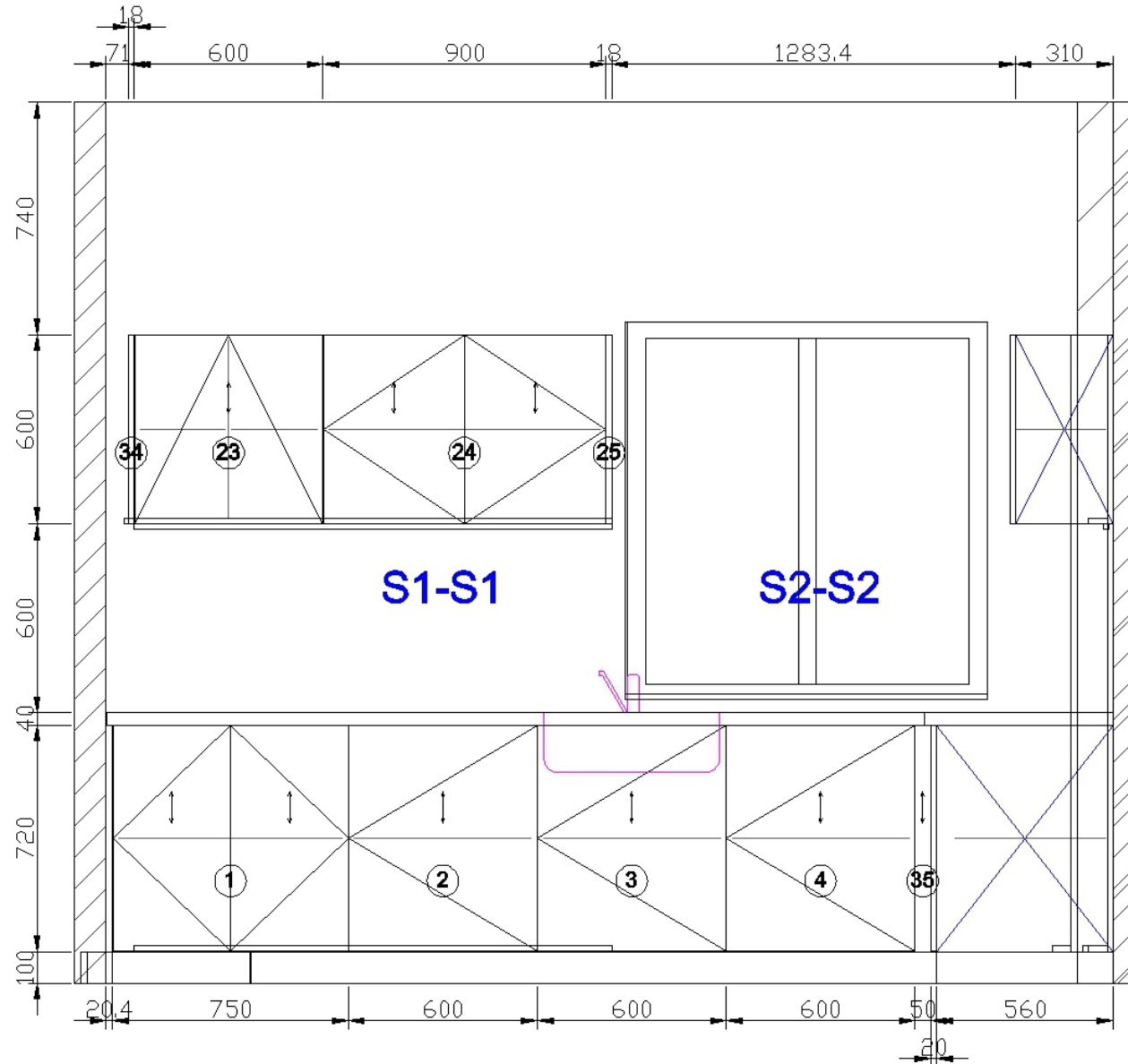
A View elevation drawing
